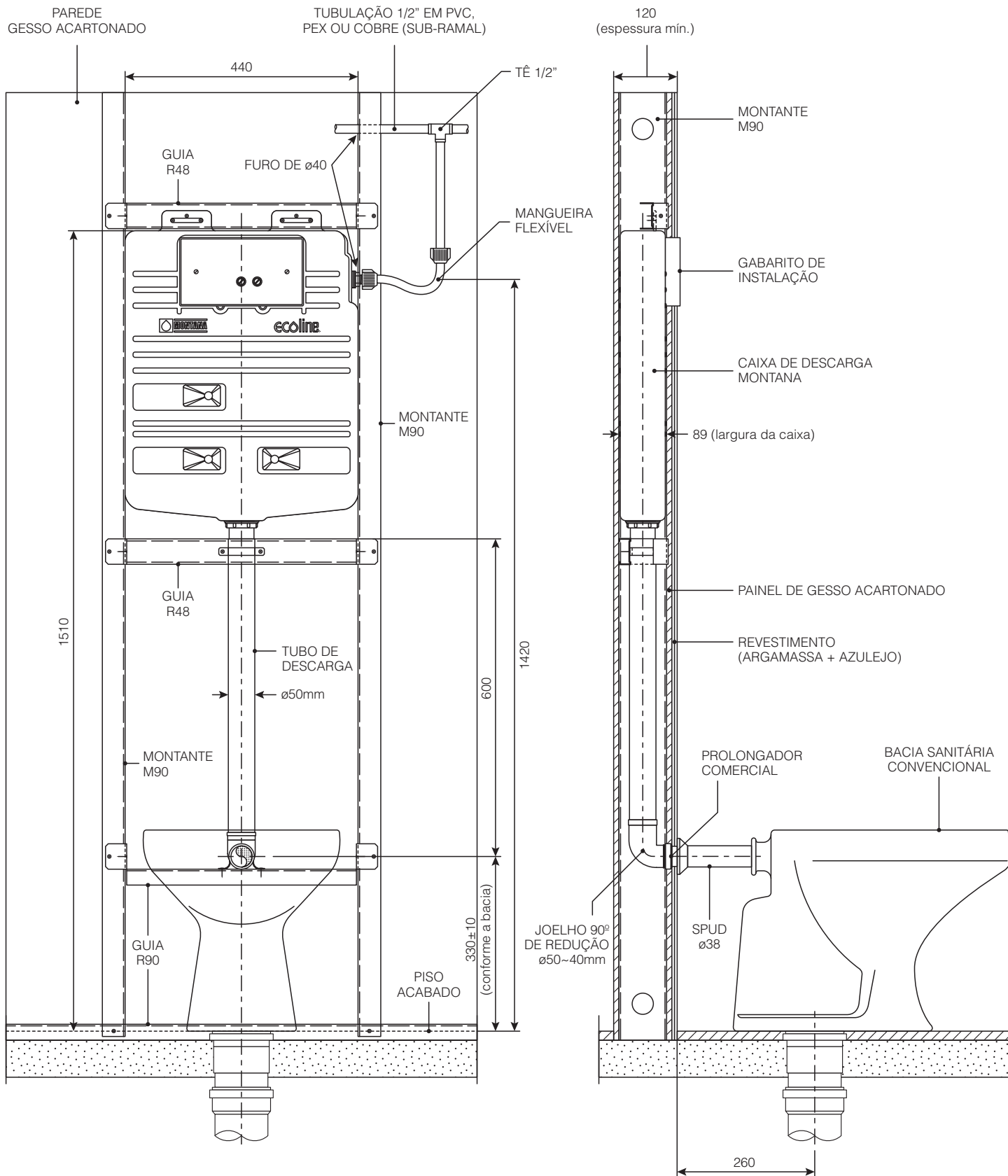
VISTA FRONTAL
